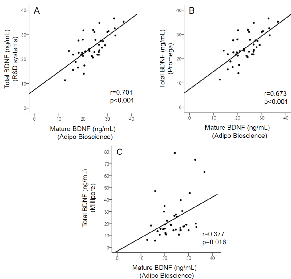
Fig. (2). Correlations between mature BDNF (Adipo Bioscience) and total BDNF (R&D System, Promega, Millipore) in human serum. (A) There was a significant correlation ( r=0.701 , p<0.001 ) between mature BDNF serum levels (Adipo Bioscience), and total BDNF serum levels (R&D Systems). (B) There was a significant correlation ( r=0.673 , p<0.001 ) between mature BDNF serum levels (Adipo Bioscience), and total BDNF serum levels (Promega). (C) There was also a significant correlation ( r=0.377 , p=0.016 ) between mature BDNF serum levels (Adipo Bioscience) and total BDNF serum levels (Millipore).
