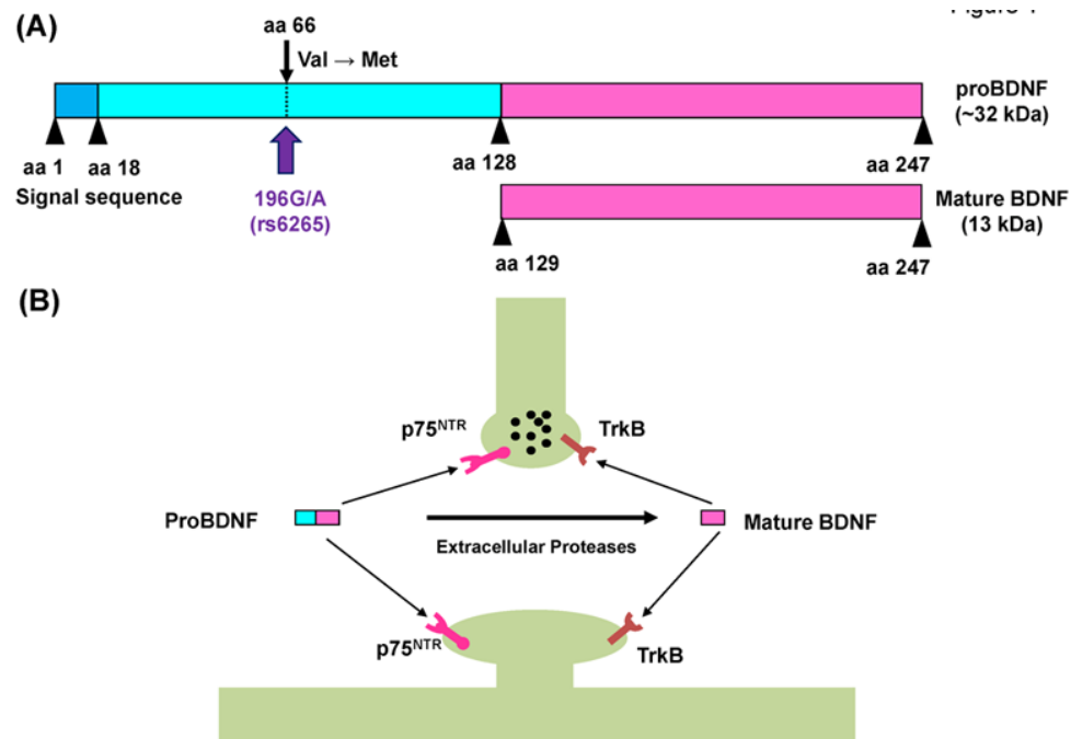
Fig. (1). (A) Structure of proBDNF and mature BDNF. Arrowheads indicate known protease cleavage sites involved in the processing of mature BDNF. The position of the single nucleotide polymorphism (rs6265, Val66Met) in the human BDNF gene is indicated by an arrow. (B) Extrasynaptic cleavage of proBDNF to mature BDNF. ProBDNF preferentially binds p75 NTR . ProBDNF is cleaved by extracellular proteases at the synapses and converted to mature BDNF. Mature BDNF preferentially binds the TrkB receptor. This figure is a modified version of previously published figures [9-11].
